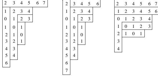
FIGURE 9. \mu_1, \mu_2, \mu_3
